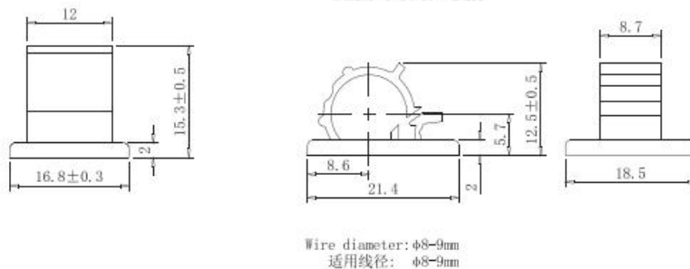
Part No. GN-11A
