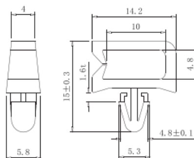
Part No. WH-A
