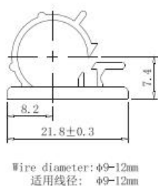
Part No. GN-10A
