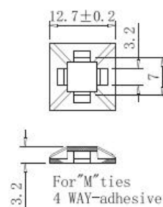
Part No. GN-2A
