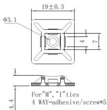
Part No. GN-3A
