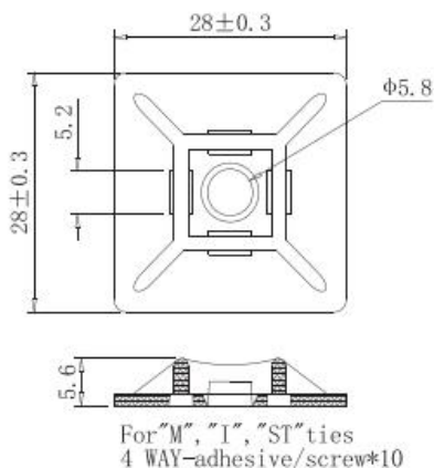
Part No. GN-4A
